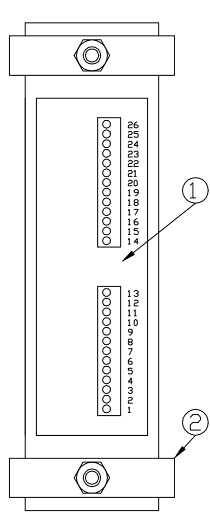
REAR
