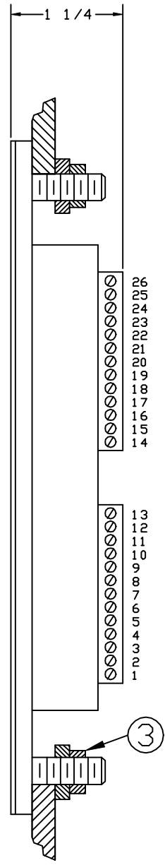
SIDE
